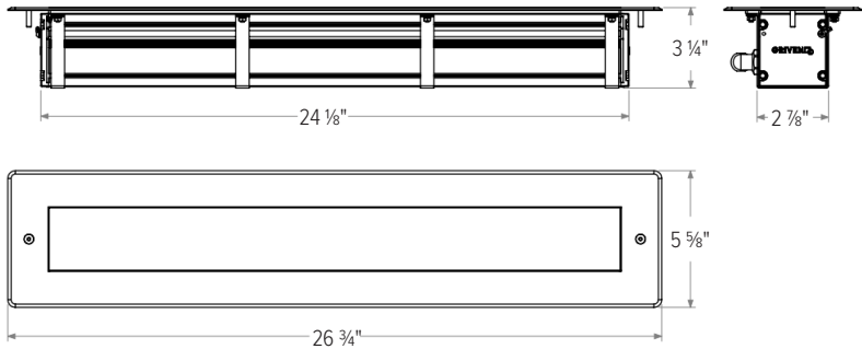
PARADE L2 RECESSED Luminaire Dimensions
