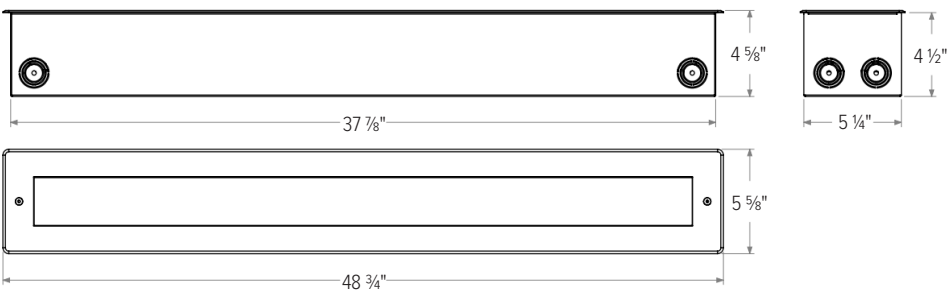
PARADE L3 RECESSED Back Box Dimensions
